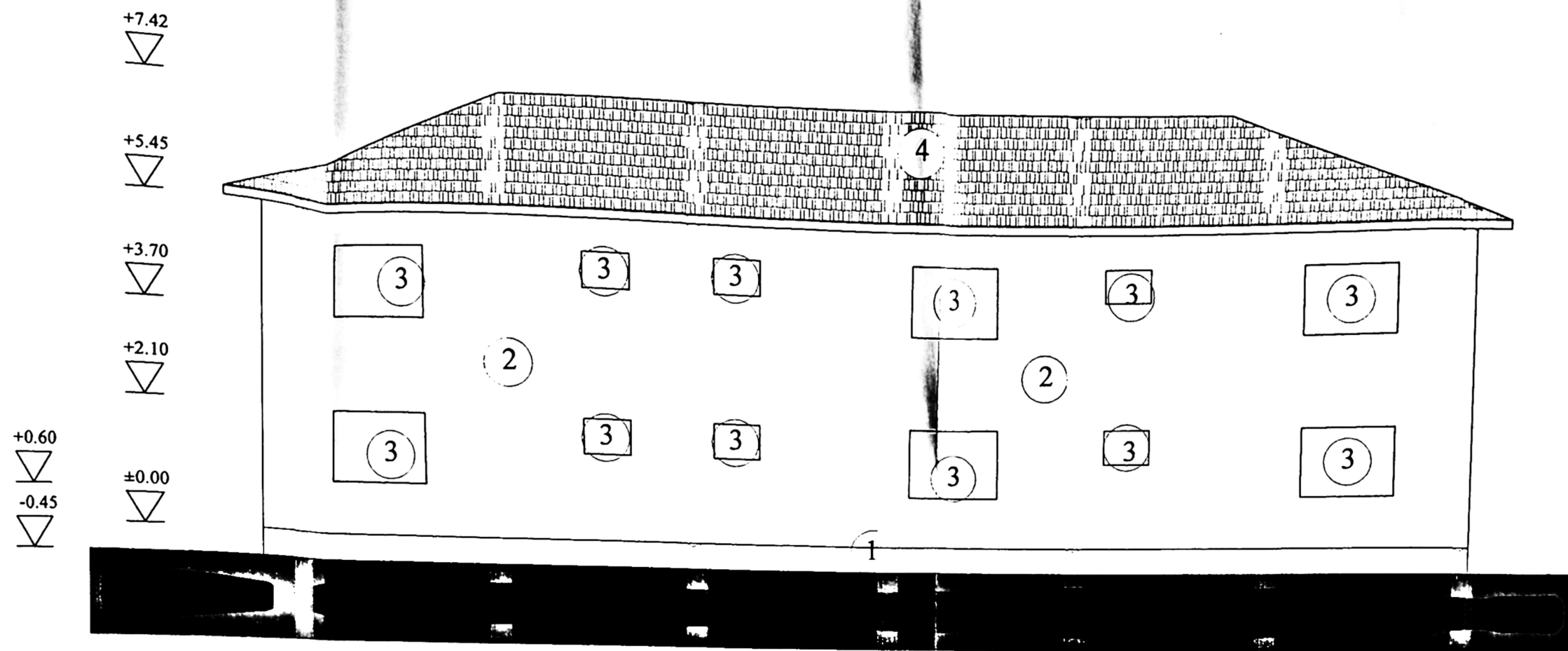
FATADA VEST
